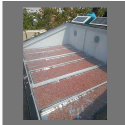
Modular Solar Dryer
