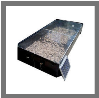
Solar Conduction Dryer
