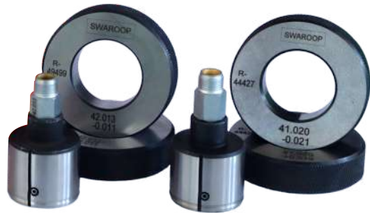
► Air Plug Gauges with setting rings
