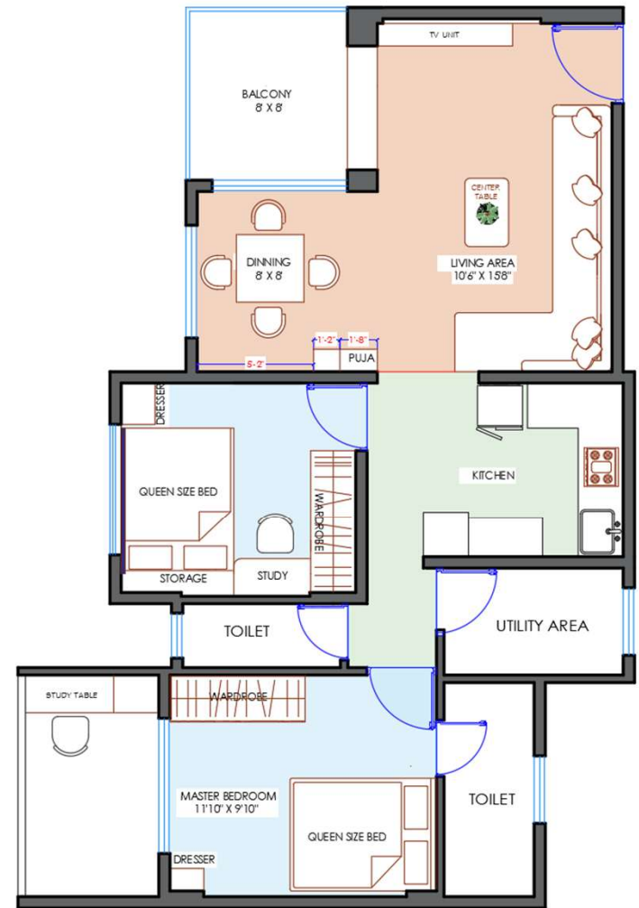
2 BHK FLOOR PLAN WITH FURNITURE LAYOUT
