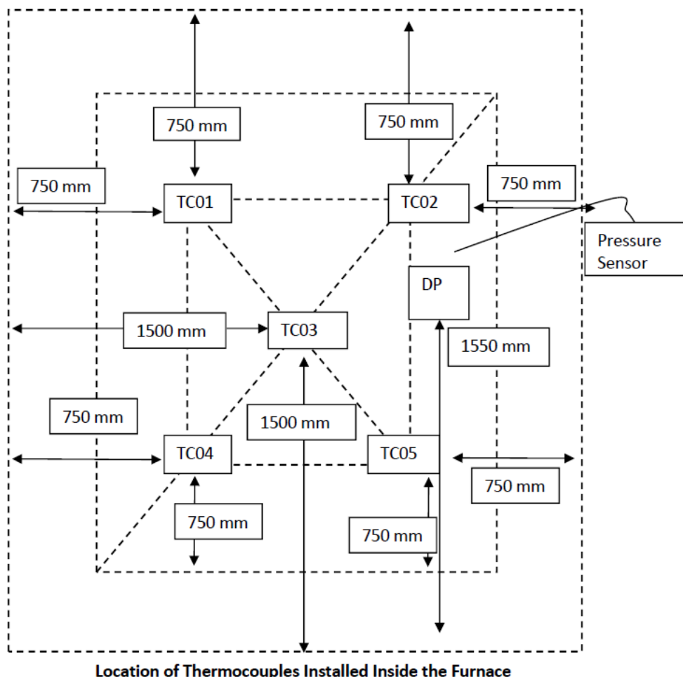
Location of Thermocouples Installed Inside the Furnace
