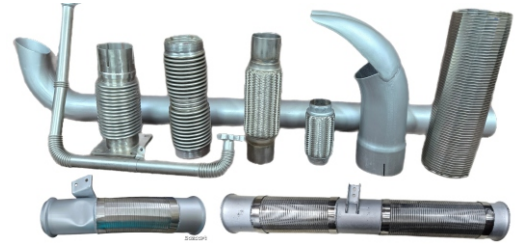
Exhaust Bellows & EGR Tubes
