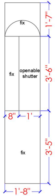
SIDE ELEVATION
