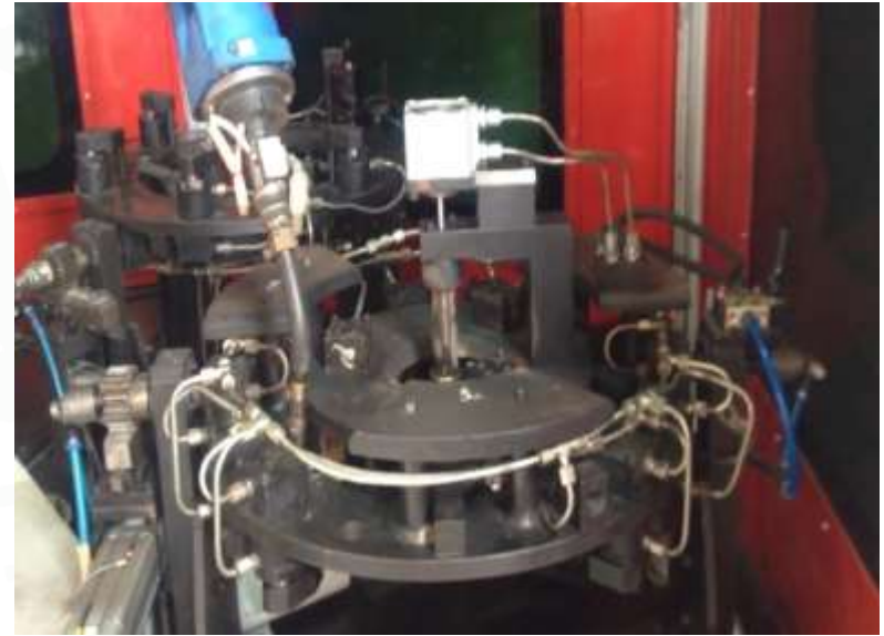
Fixture tilts 180° for Bottom side Welding
