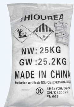
Thiourea
