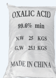
Oxalic Acid
