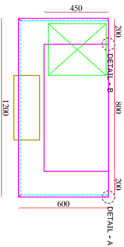
RECEPTION TABLE PLAN
