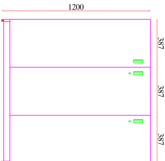
OUTER VIEW
