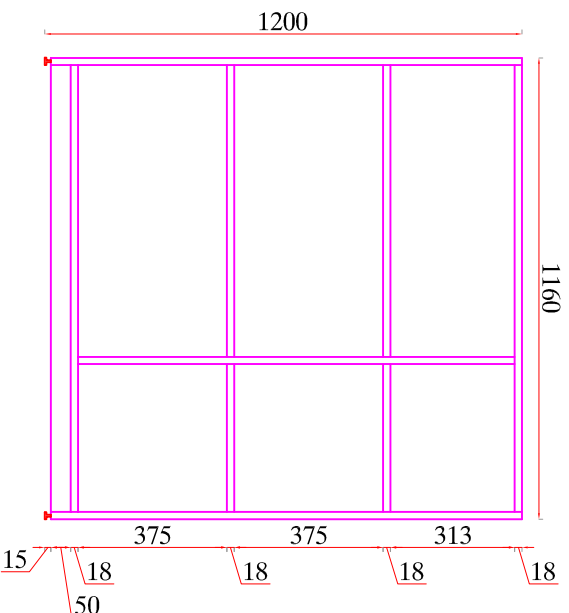
INNER VIEW
