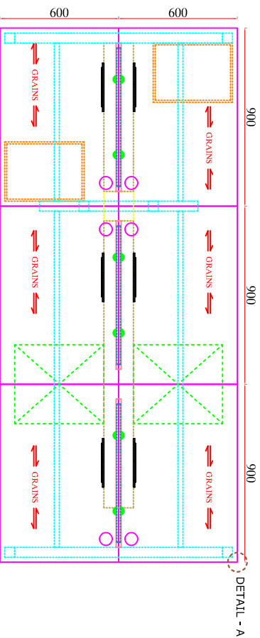
SHARING WORKSTATION PLAN
