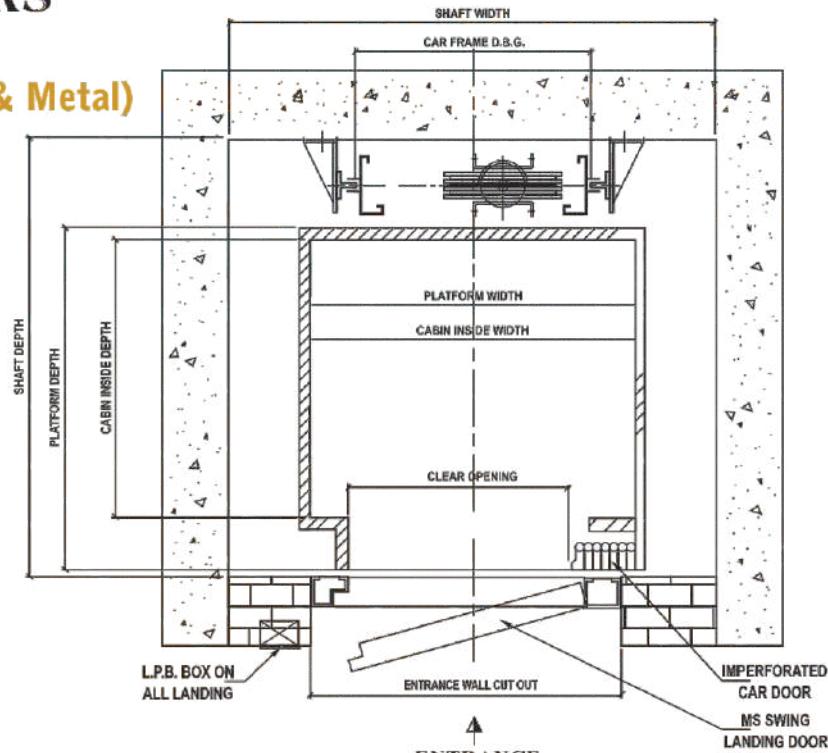
ENTRANCE CROSS SECTION PLAN OF ELEVATOR SHAFT
