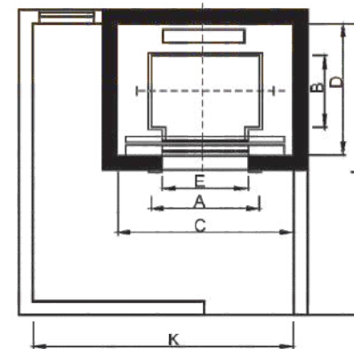
MACHINE ROOM & HOISWAY PLAN
