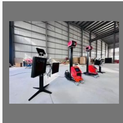
Truck Wheel Alignment Machine
