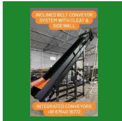
Cleated Belt Incline Conveyors
