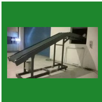
Truck Loading Conveyor System
