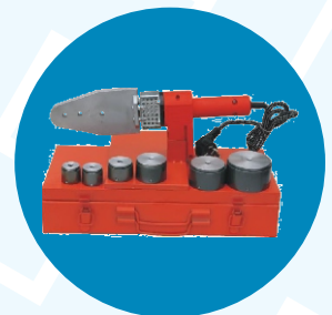
Welding Machine Die Mfg Range : 20 mm to 160 mm
