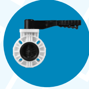
Butter Fly Valves - Manual Operated Manufacturing Range : 2" to 8" M.O.C. : PP / ISO PP / PPH / PVDF
