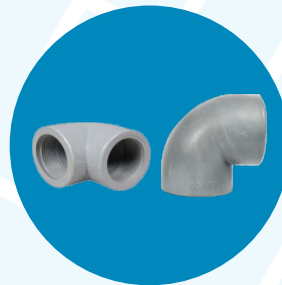
Socket Bend ( Plain ) Mfg Range : 20 mm OD to 160 mm OD Socket Bend ( Threaded ) Mfg Range : 20 mm OD to 63 mm OD
