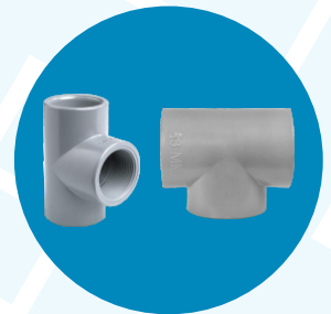
Socket Tee ( Plain ) Mfg Range : 20 mm OD to 160 mm OD Socket Tee ( Threaded ) Mfg Range : 20 mm OD to 63 mm OD
