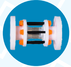
Sight Glass Manufacturing Range : 1/2" to 12" M.O.C. : PP / ISO PP / PPH / PVDF
