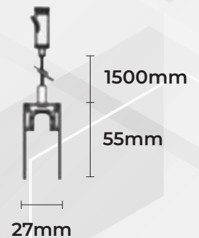
Surface mounted track (suspension)
