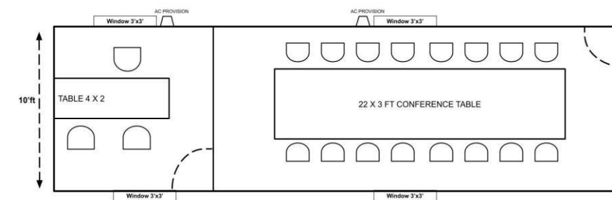
FIRST FLOOR CONFERENCE CABIN 40 X 10
