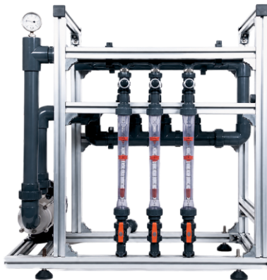
3 Channel Model ( 2 Fertilizer + 1 Acid Channel )
