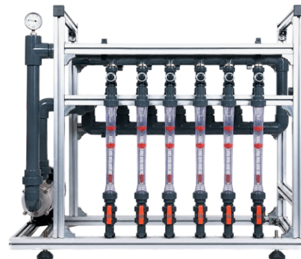
6 Channel Model ( 5 Fertilizer + 1 Acid Channel )
