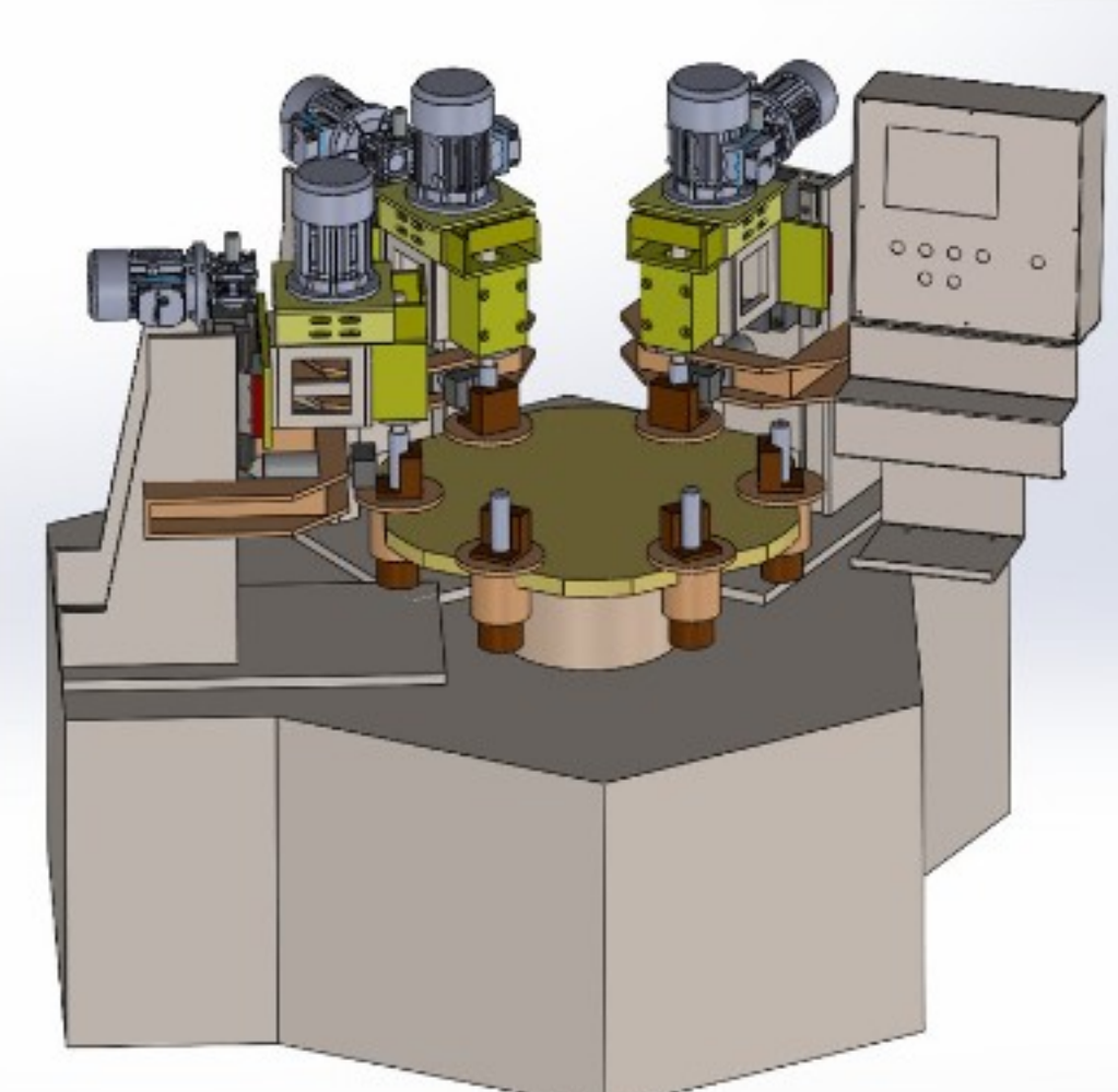
Automatic Rotary Indexing Table Facing, Drilling & tapping Machine
