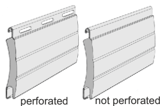
Aluminium Profile PA-45 Available colours – 18
