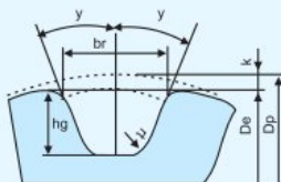
Dimension of T type pulley (mm)
