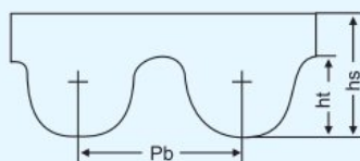
HTD Arc tooth
