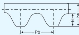
STPD/STS Arc tooth
