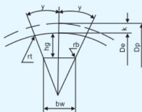
Dimension of HTD type pulley (mm)
