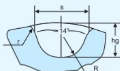
Dimension of T type pulley (mm)
