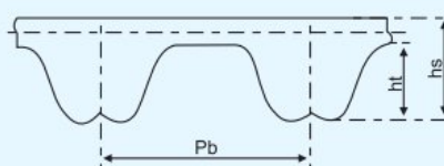
RPP/HPPD Arc tooth
