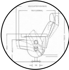
PUSH BACK MECHANISM WITH 45 DEGREE RECLINE
