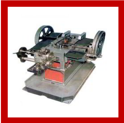
High Speed Double Stroke Header Machine
