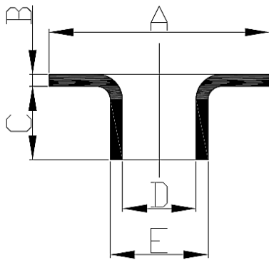
NOZZLE BUSH
