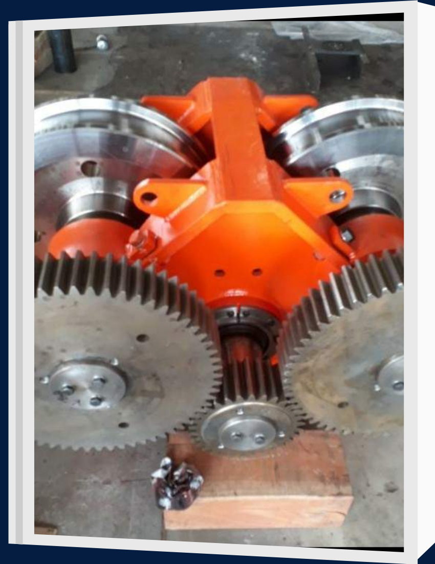
DRIVE BOGGY
