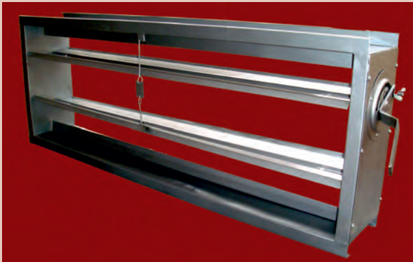
Fire Damper with Fusible Link
