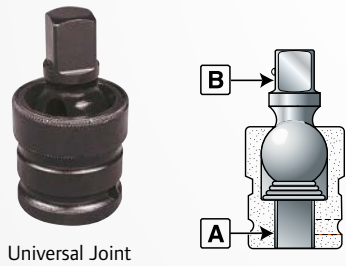
Universal Joint
