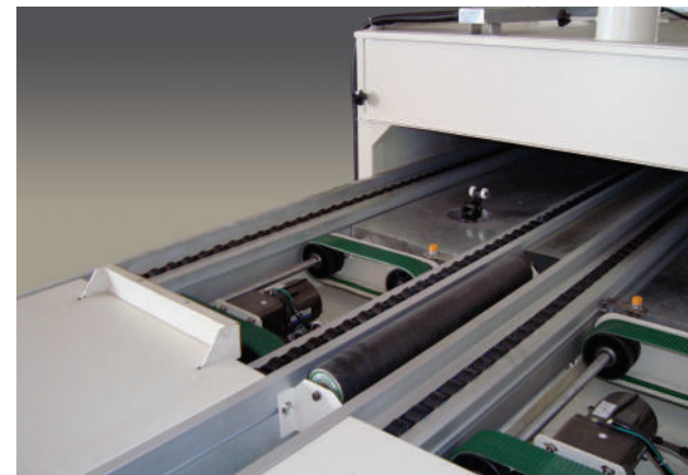
Free Flow Conveyor with Pallet Transfer
