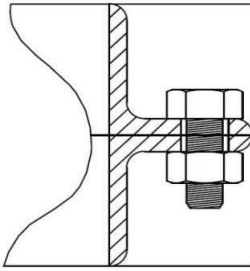
Angle Base / Angle Hold down Welded Installation (Includes Hex Bolt & Nut fasteners)
