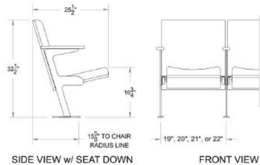
SIDE VIEW w/ SEAT DOWN
