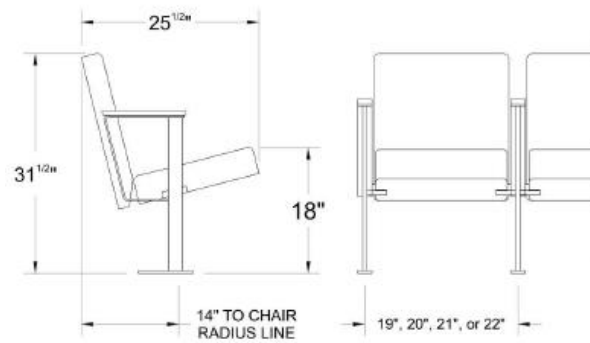
SIDE VIEW w/ SEAT DOWN
