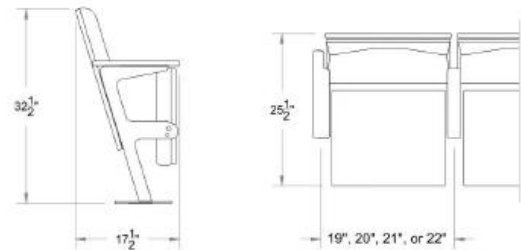
SIDE VIEW w/ SEAT UP
