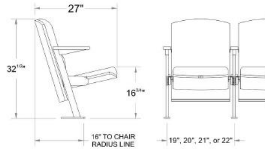
SIDE VIEW w/ SEAT DOWN
