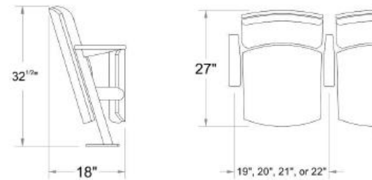
SIDE VIEW w/ SEAT UP
