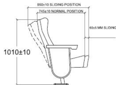
SIDE VIEW SEAT UP
