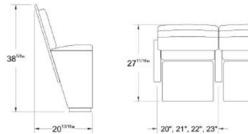
SIDE VIEW w/ SEAT UP
