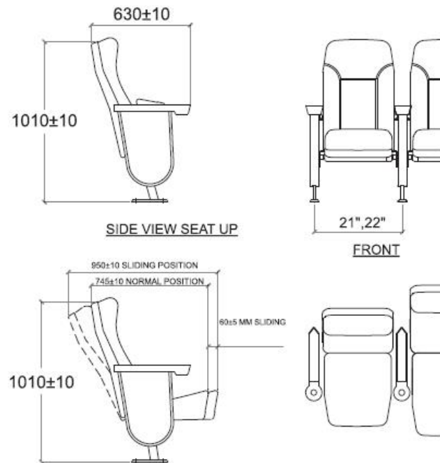
SIDE VIEW SEAT SLIDING
