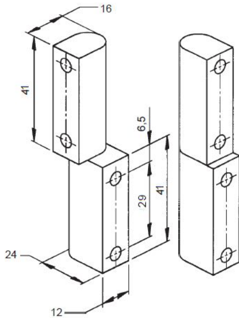
Panel Hinge APH 880
