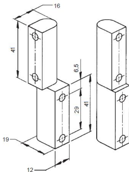
Panel Hinge APH 820
