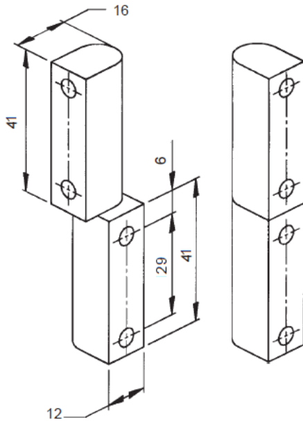
Panel Hinge APH 650
