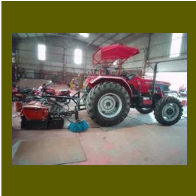
Tractor Mounted Hydraulic Road Sweeper
