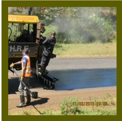
Bitumen Sprayer
