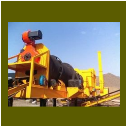
Asphalt Drum Mixing Plant
